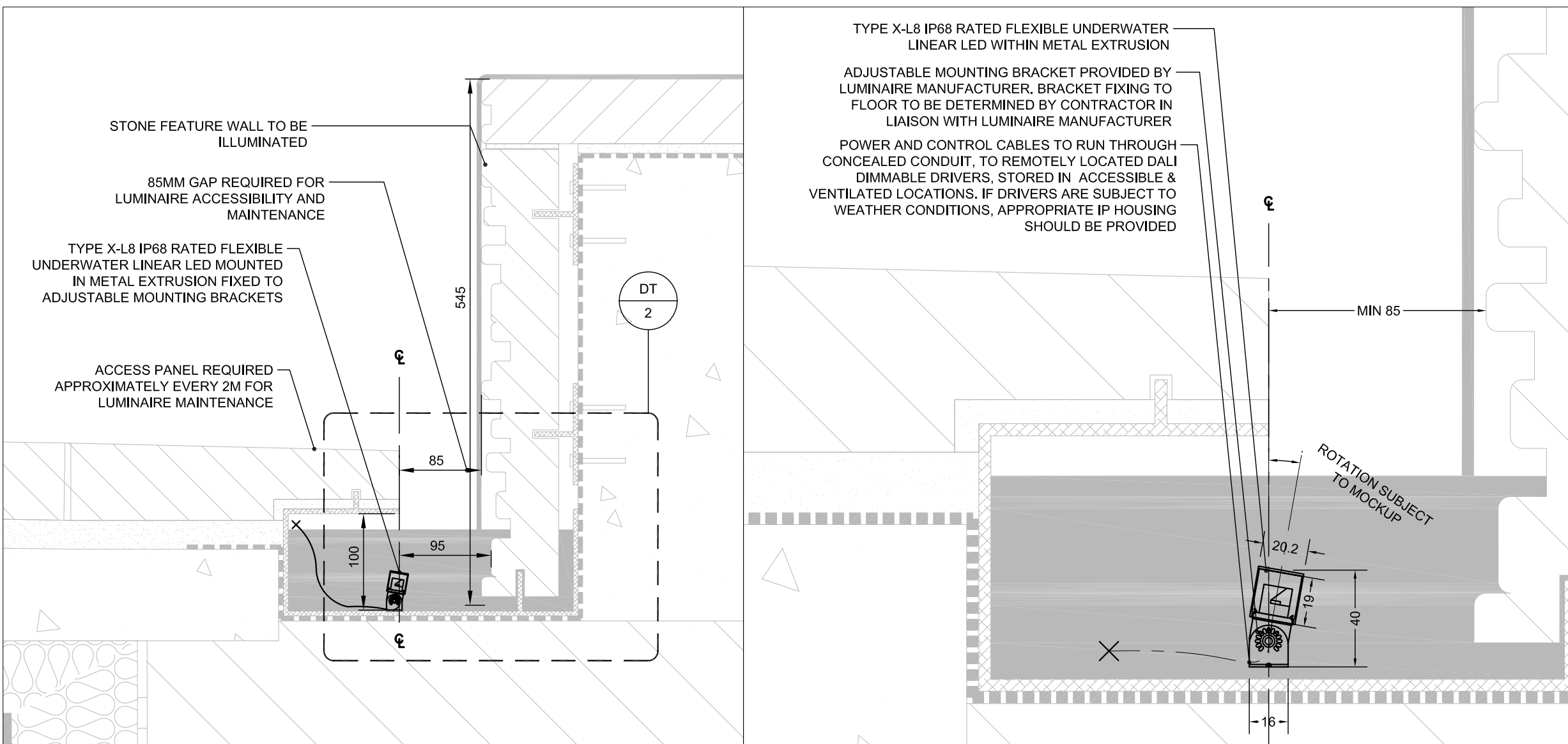
2003 - 1 - WATER FEATURE - SCALE 1:5
