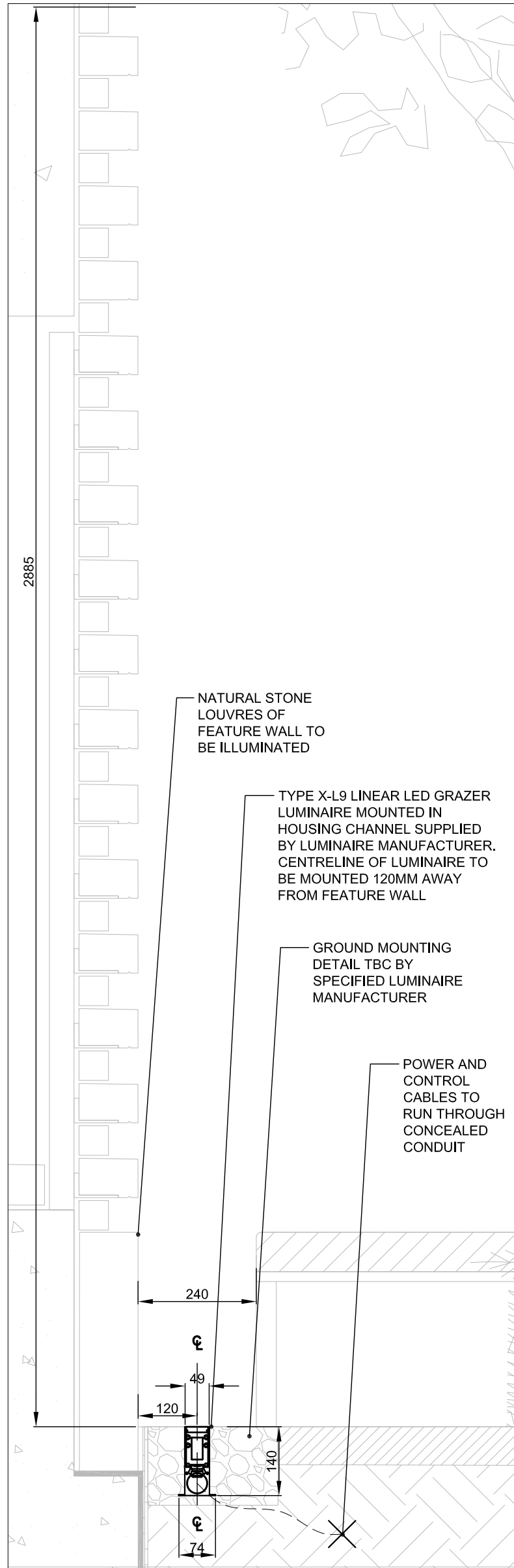
2005 - 1 - FEATURE WALL - SCALE 1:10
