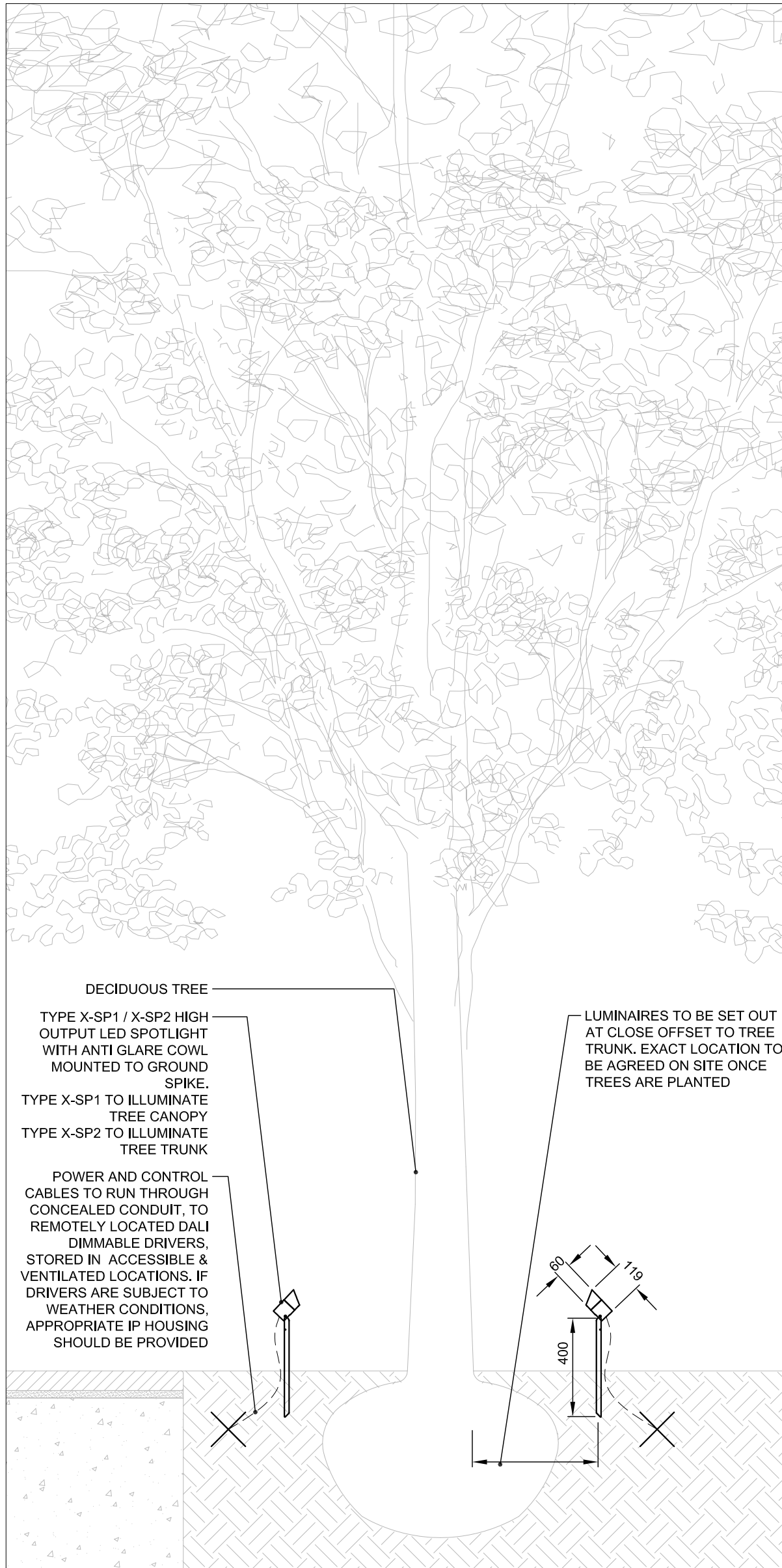
2004 - 1 - TREES - SCALE 1:20
