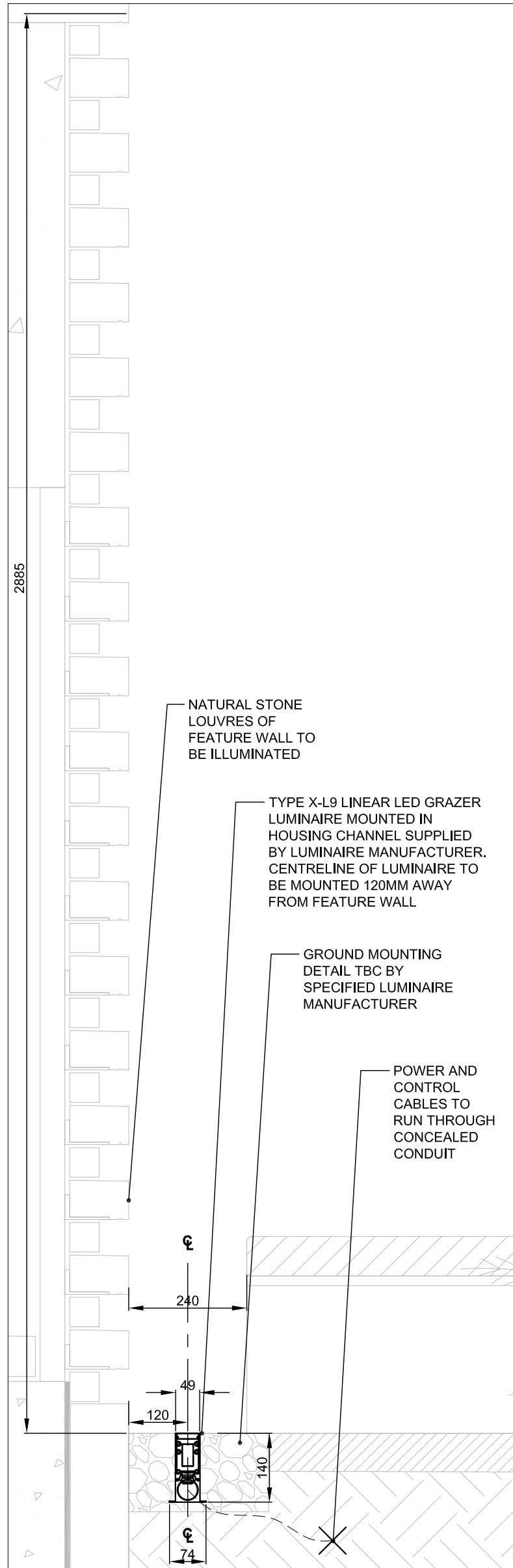
2005 - 2 - FEATURE WALL - SCALE 1:10
