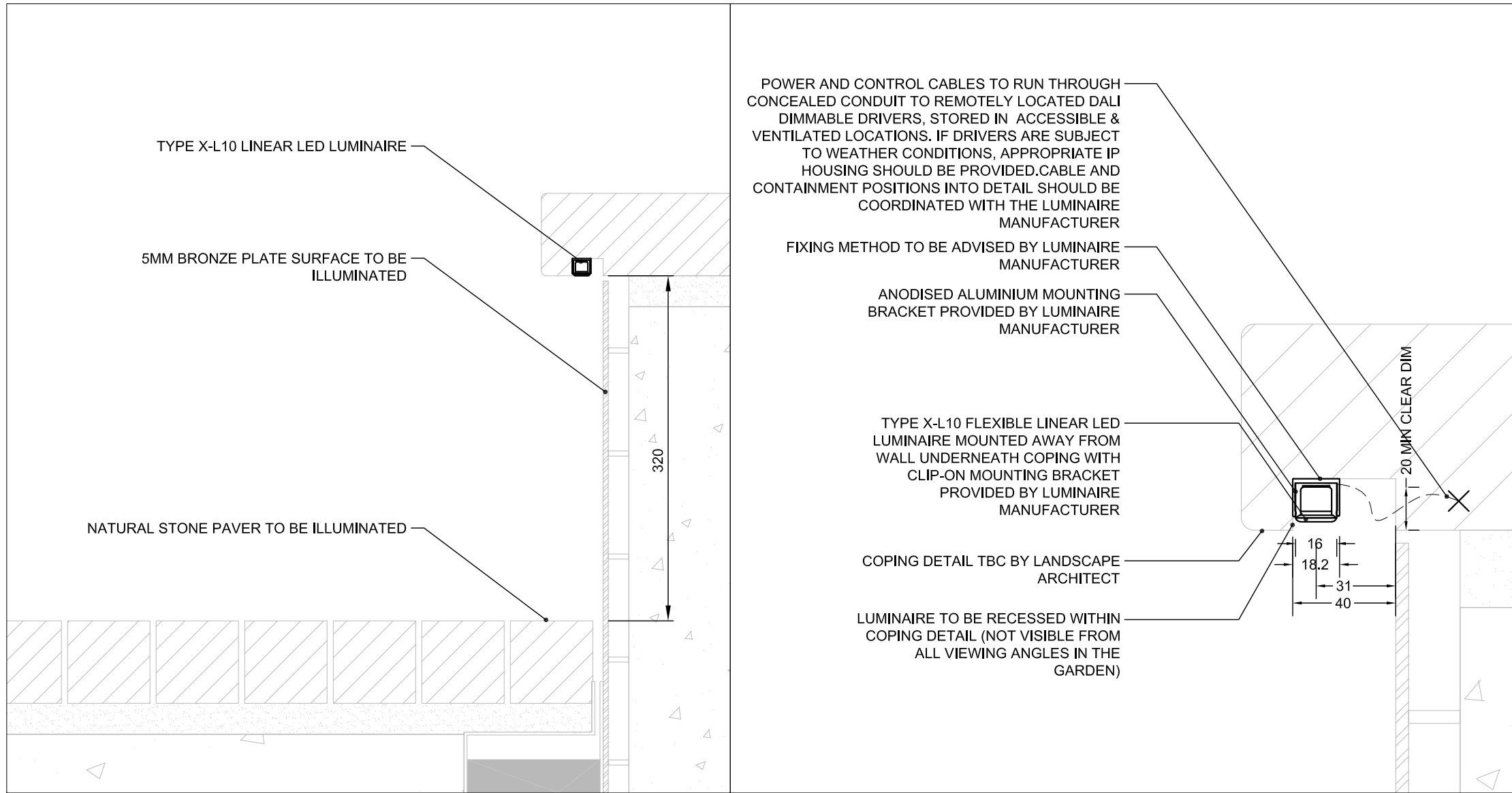
2001 - 1 - SEATING WALL - SCALE 1:5
