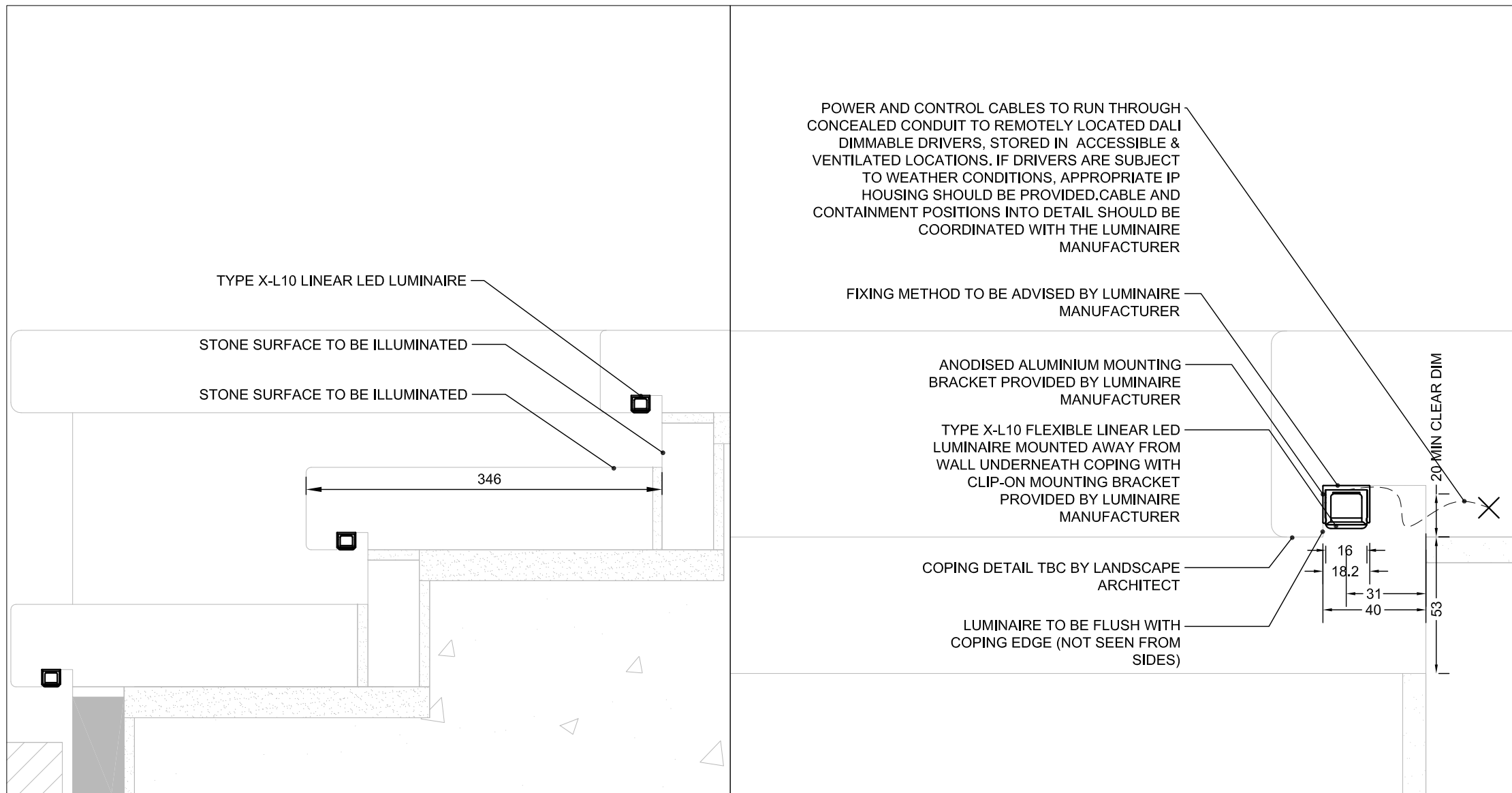
2002 - 1 - STEPS - SCALE 1:5
